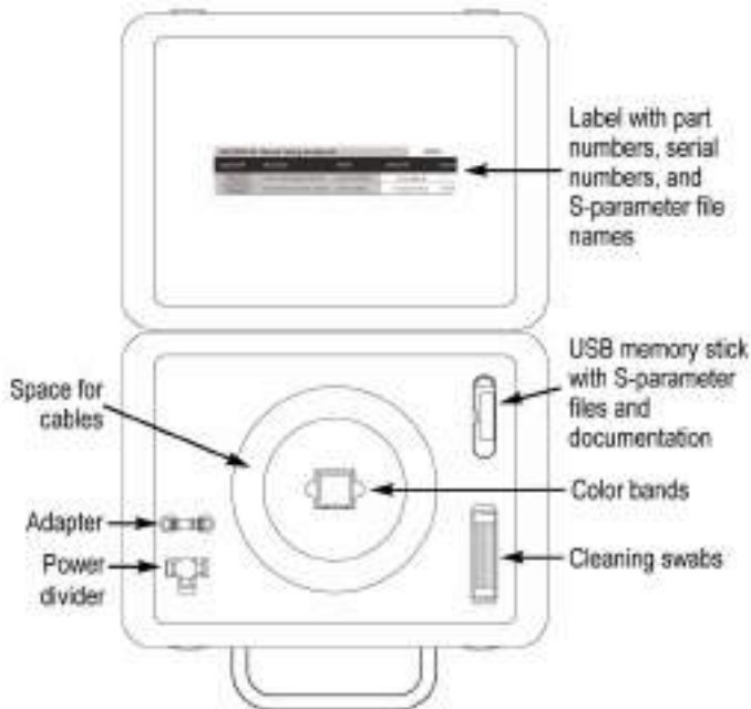
DPO7RFK3-1.85 mm deskew kit.
