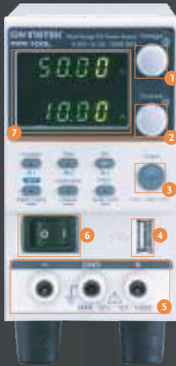
PFR-100L Front Panel
