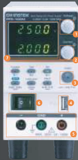
PFR-100M Front Panel
