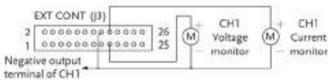
External Voltage Monitor of the Output
