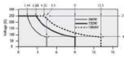
PSW 250V Series Operating Area
