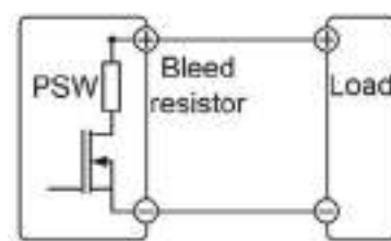
PSW-Series Built-in Bleed Resistor
