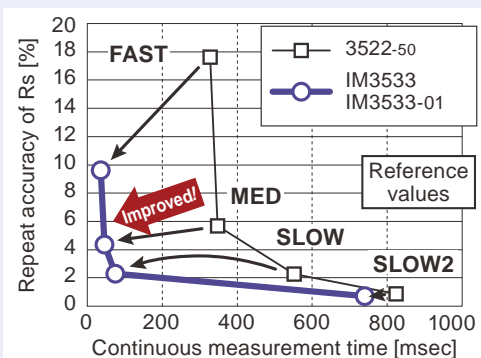
Continuous measurement time and repeat accuracy of Rs in C-D + ESR continuous measurement at 100kHz (Sample: aluminum electrolyte capacitor 1.5 \mu F)
