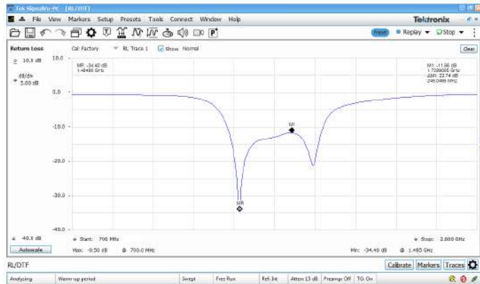
Return loss of a bandpass filter measured from 700 MHz to 2.6 GHz. Markers have been placed at 1.48 GHz (-34.4 dB return loss) and at 1.73 GHz (-11.68 dB return loss), indicating the best and worse match in the passband of the filter.
