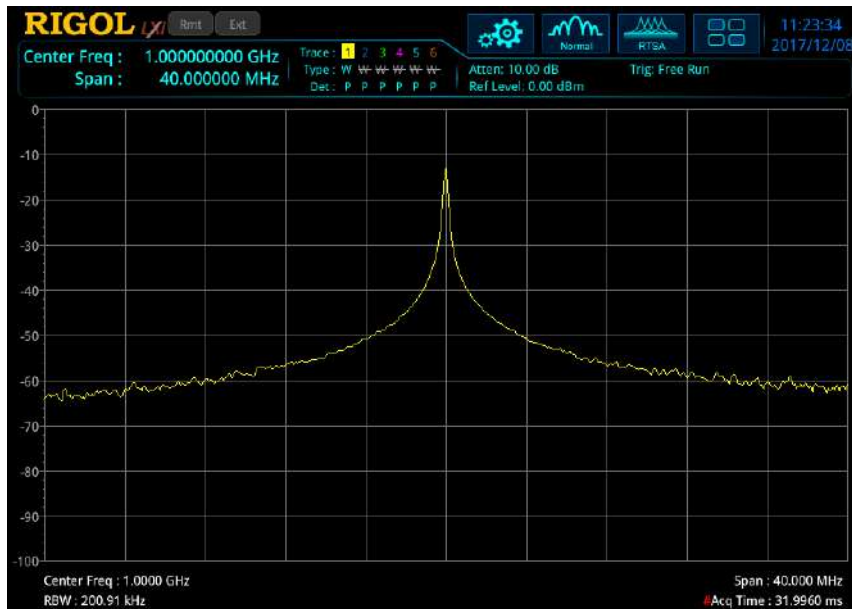
Figure 3-1 Normal View
