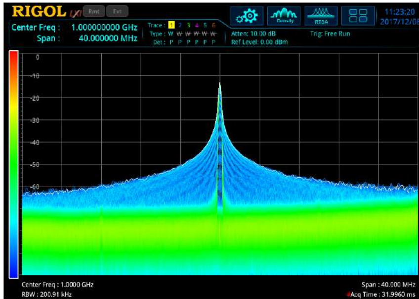
Figure 3-2 Density View
