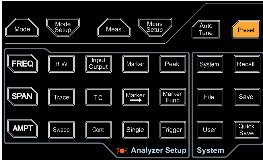
Figure 1-5 Function Keys
