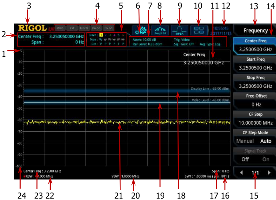
Figure 1-9 User Interface
