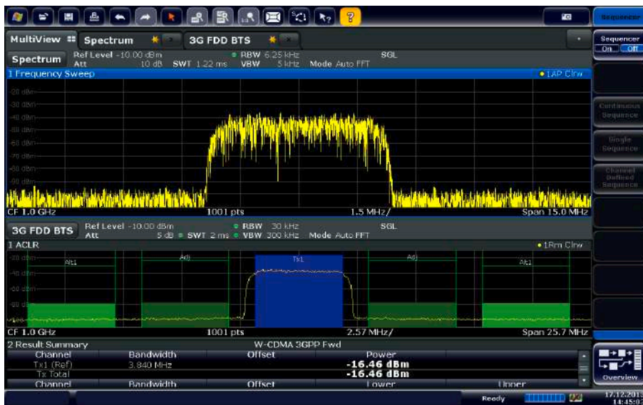
Amplifier measurement showing numerical results and graphical representation of AM/AM and AM/PM distortion
