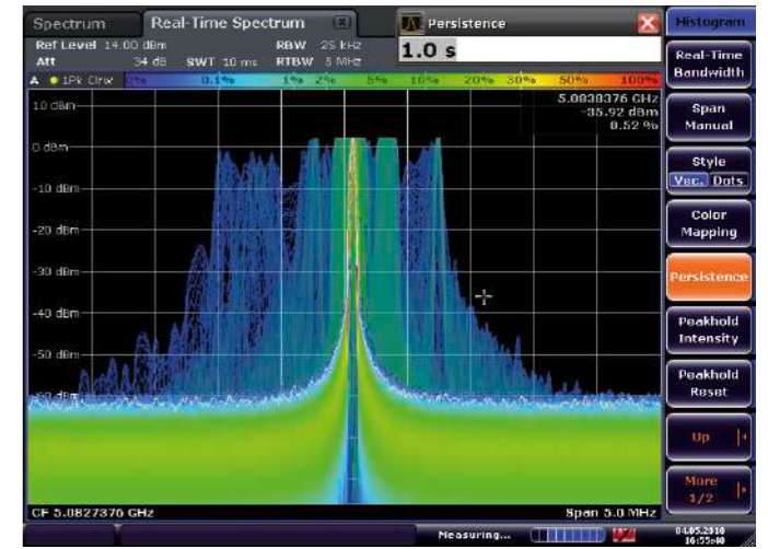
Transient response of a VCO for WLAN applications in persistence mode.
