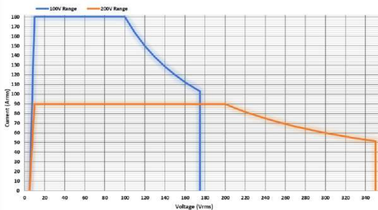
ASR-6600-18 AC Mode Output Operating Area
