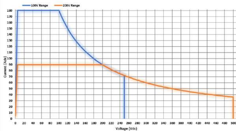
ASR-6600-18 DC Mode Output Operating Area
