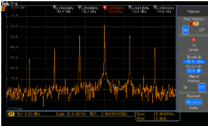
Automated peak markers identify critical information at a glance. As shown here, the five highest amplitude peaks that meet the threshold and excursion criteria are automatically marked along with the peak's frequency and amplitude.
