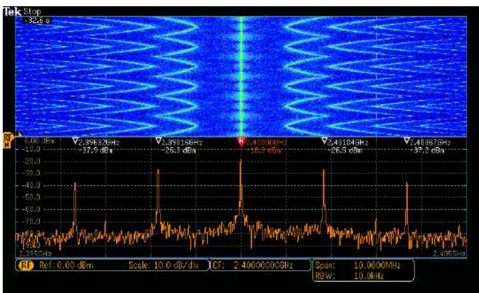
Spectrogram display illustrates slowly moving RF phenomena. As shown here, a signal that has multiple peaks is being monitored. As the peaks change in both frequency and amplitude over time, the changes are easily seen in the Spectrogram display.
