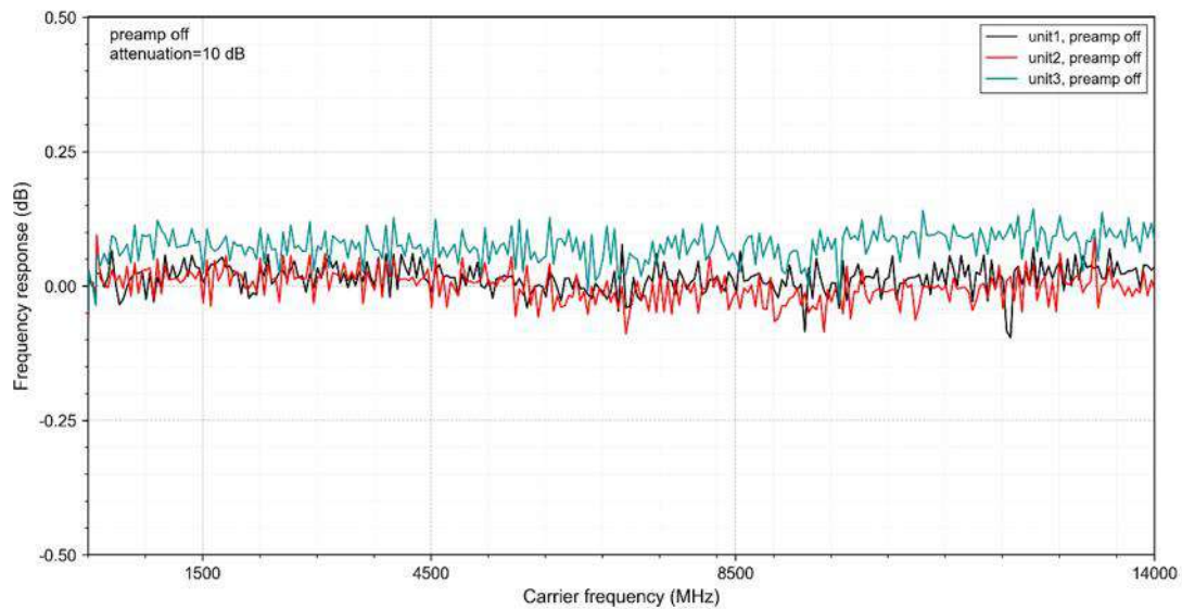
Frequency Response (attenuation = 10 dB, PA off)
